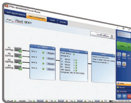
Ethernet multiclients
